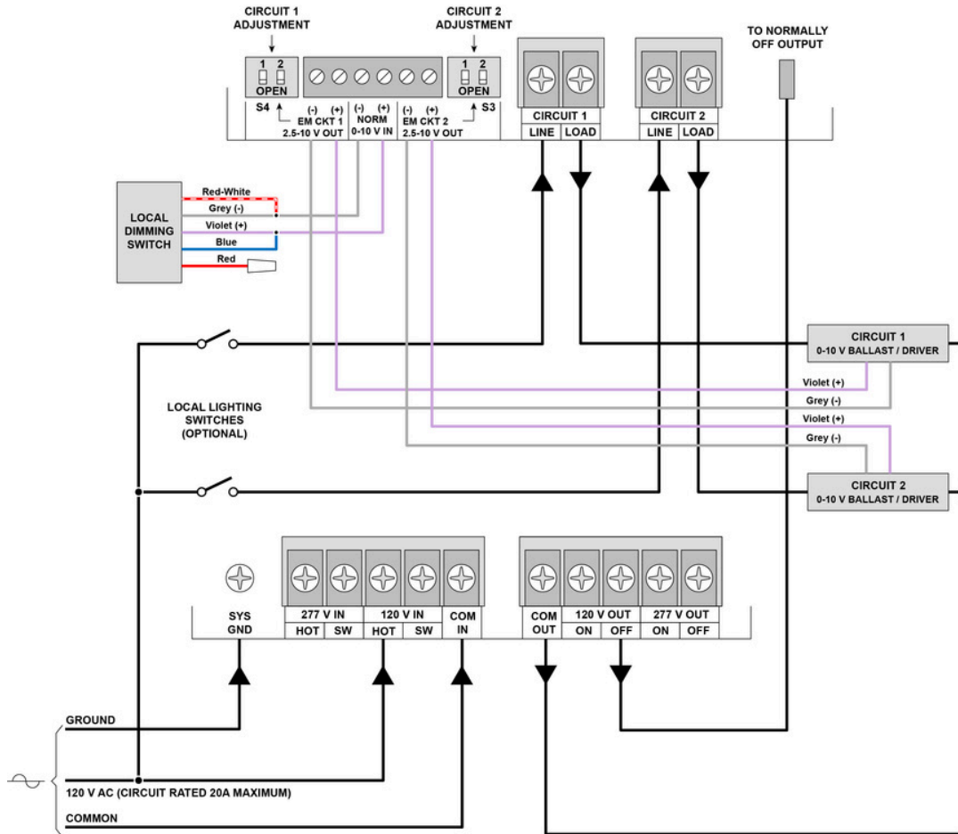
DIMMING OPTIONS, 120V OPERATION
