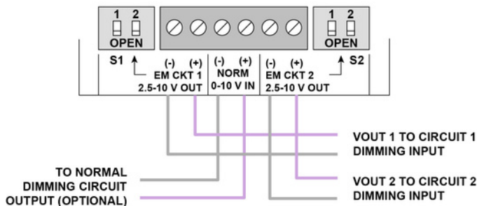
DIMMING OPTIONS CONTROL WIRING
