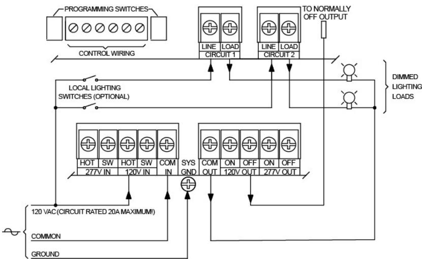
G) DIMMING OPTION, 120V OPERATION
