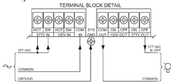
I) NORMALLY OFF LOADS
