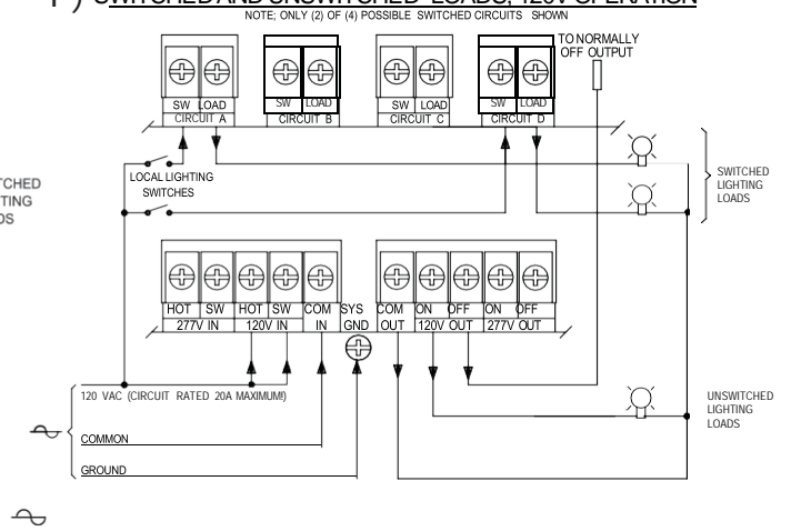
F) SWITCHED AND UNSWITCHED LOADS, 120V OPERATION
