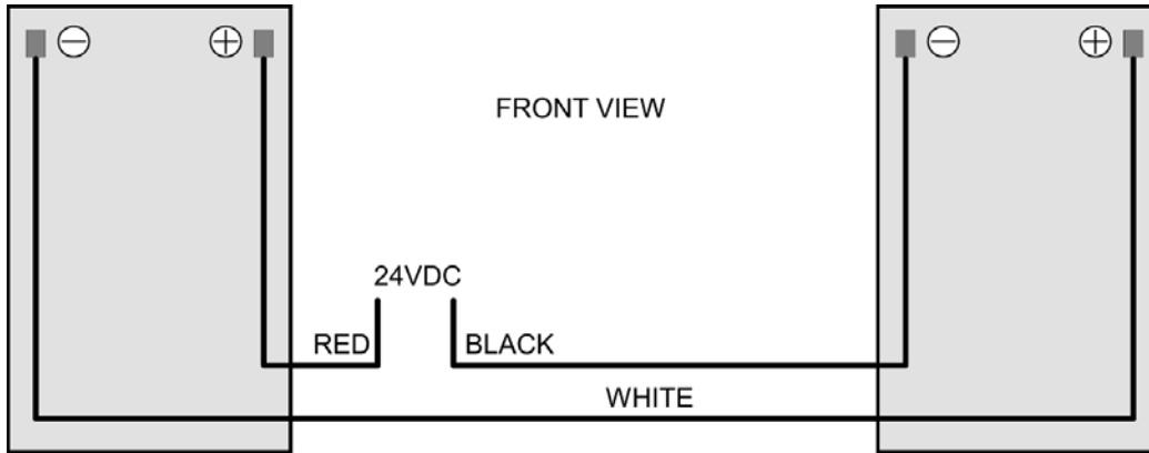
Wiring Diagram 2
