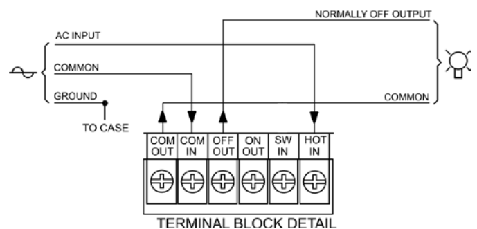
Diagram 4. SWITCHED LOADS
